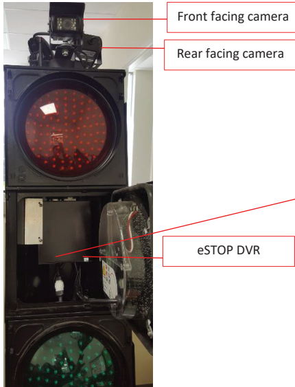
Figure 1. eSTOP Camera and DVR
